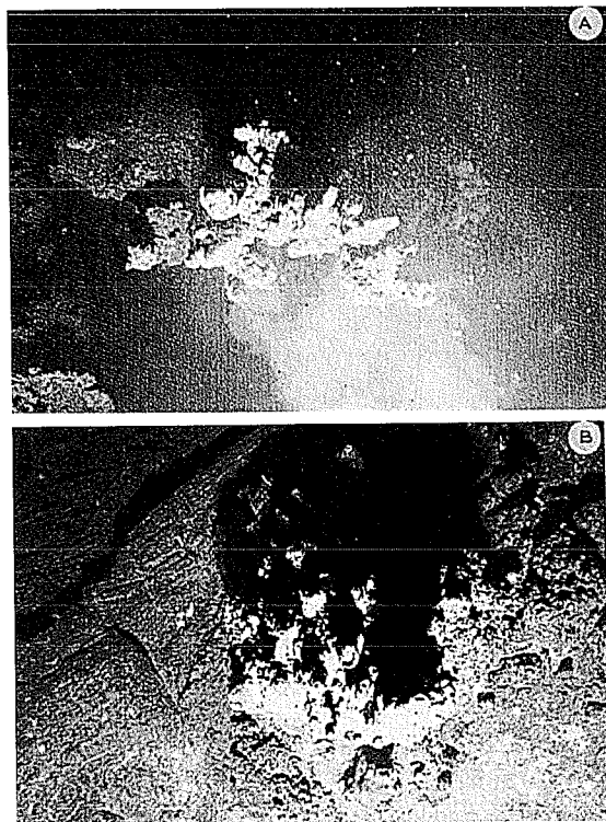
Fig. 6. A. Top view of an active black smoker edifice along the base of the west wall of the ASC in Segment B2 near 9°45'N. Electronic Still Camera (ESC) image, depth 2540 m, altitude = 7.0 m, heading 350° (towards top of image). Horizontal width of image is ~ 4 m. Note “smoke” plume which is wafting from the chimney spires. Edifice is ~ 7 m high and ~ 2 m wide near the top; note that several smaller chimneys have coalesced to form the top of the edifice. B. Top view of inactive sulfide edifice near the east wall of the ASC in Segment C near 9°41'N. Electronic Still Camera (ESC) image, depth 2560 m, altitude = 8.0 m, heading 350° (towards top of image). Horizontal width of image is ~ 4.8 m, image area = 15.6 m 2 . Edifice is ~ 6 m high and ~ 2.2 m wide near the top; note numerous small chimneys which extend upward from the top of edifice. The edifice appears to be a complex structure created by coalescence of the smaller chimneys.
