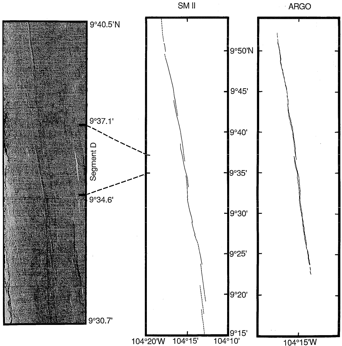
Fig. 4. EPR plate boundary configuration in the ARGO survey area. On left, blow-up of Sea MARC II sonar record between approximately 9°30' and 42' N showing paired black acoustic reflectors and white shadows characteristic of a well-developed ASC. In middle, plate boundary determined from Sea MARC II (SM II) sonar data, 9°54'–15' N, from Macdonald et al. [29]. The presence of the ASC is denoted by a solid line; the dashed line shows where the axial zone appears as a discontinuous, “fuzzy” trace in the Sea MARC II records. On right, ASC configuration determined from ARGO sonar records. Width of the ASC is measured across the top of this feature between the outermost bounding walls. Agreement between Sea MARC II and ARGO delineation of the ASC is excellent considering the difference in resolution and areal coverage for the two systems.
